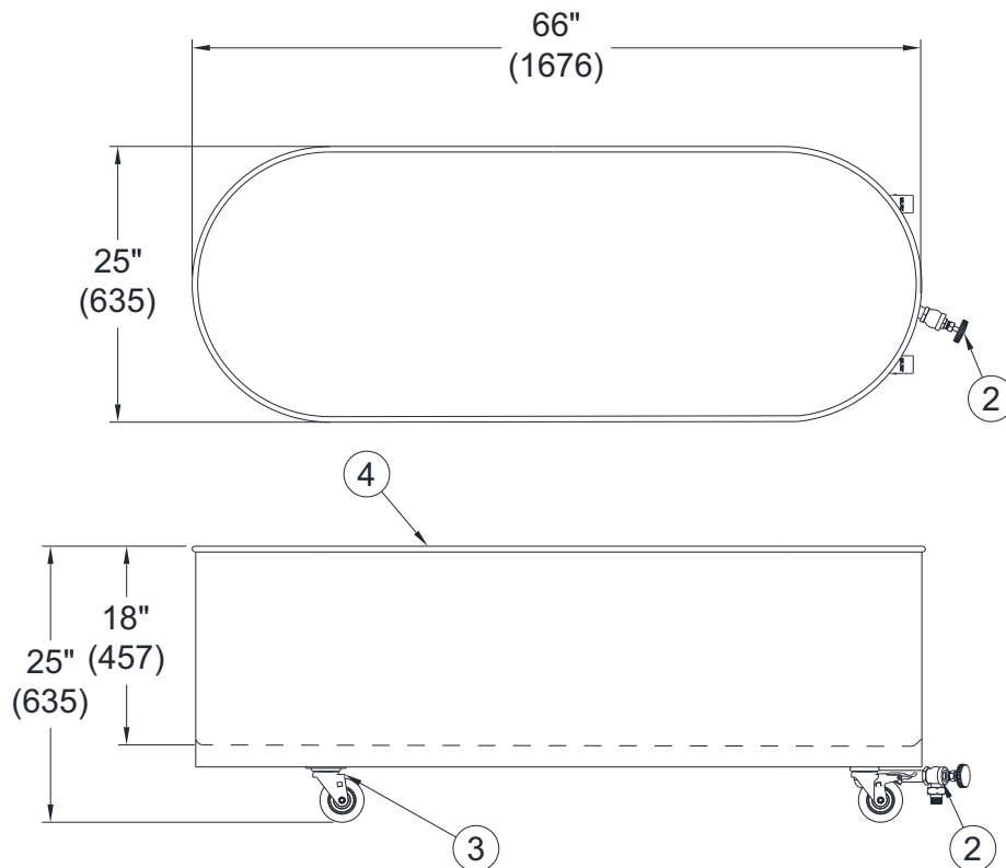
MOBILE 105-L-M-TO SERIES COLD TANK
